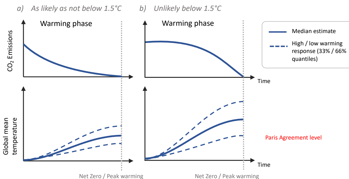
Figure 1: Stylised CO 2 emissions and warming trajectories for classification from Table 1. a) as likely as not below 1.5°C pathways and b) unlikely below 1.5°C pathways
